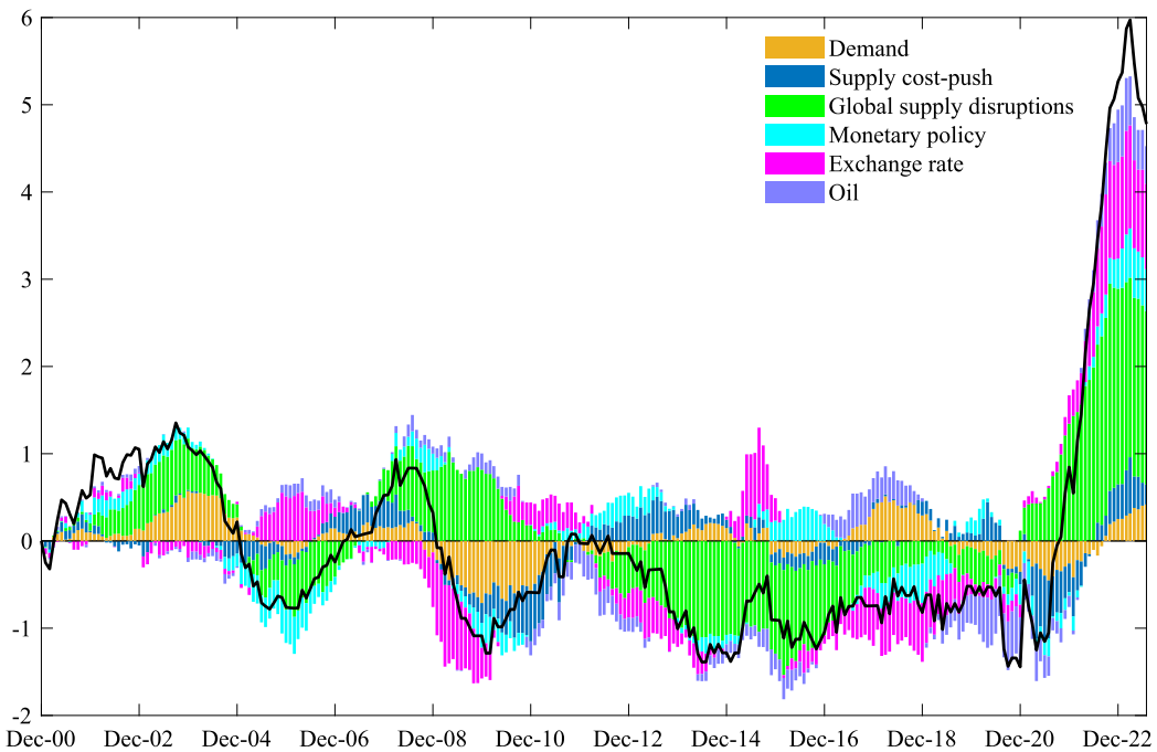
Fig. 3.6. Historical shock decomposition of euro area core inflation.
