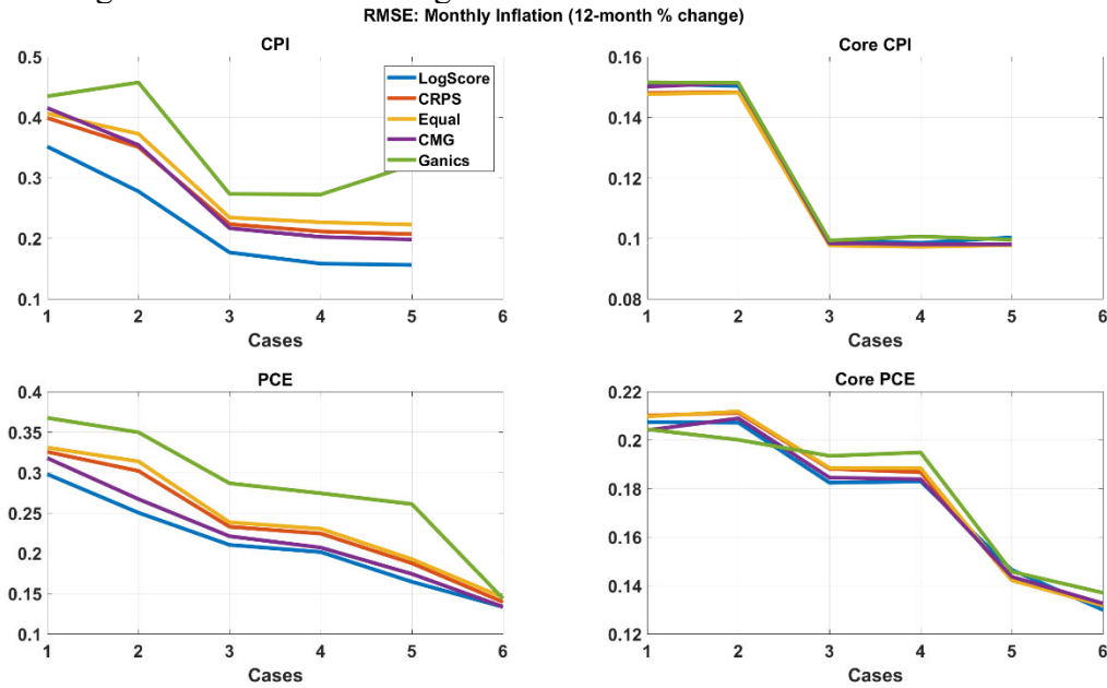
Figure 5: Point Nowcasting Performance across Grand Combinations
