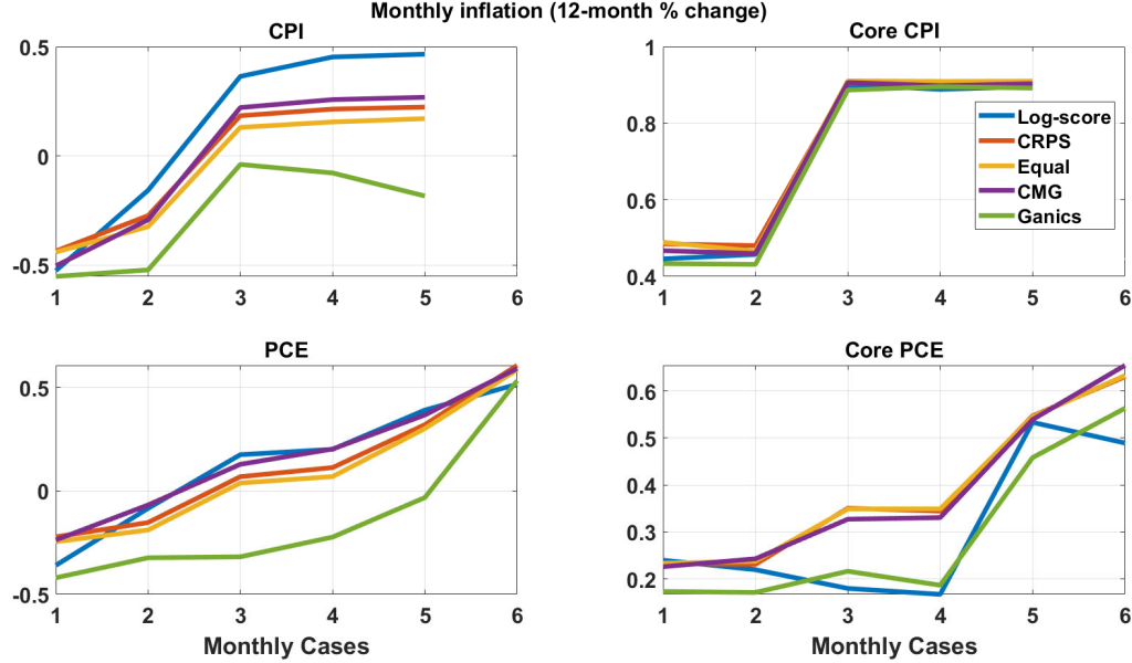
Figure 4: Density Performance Comparisons across Grand Combinations
