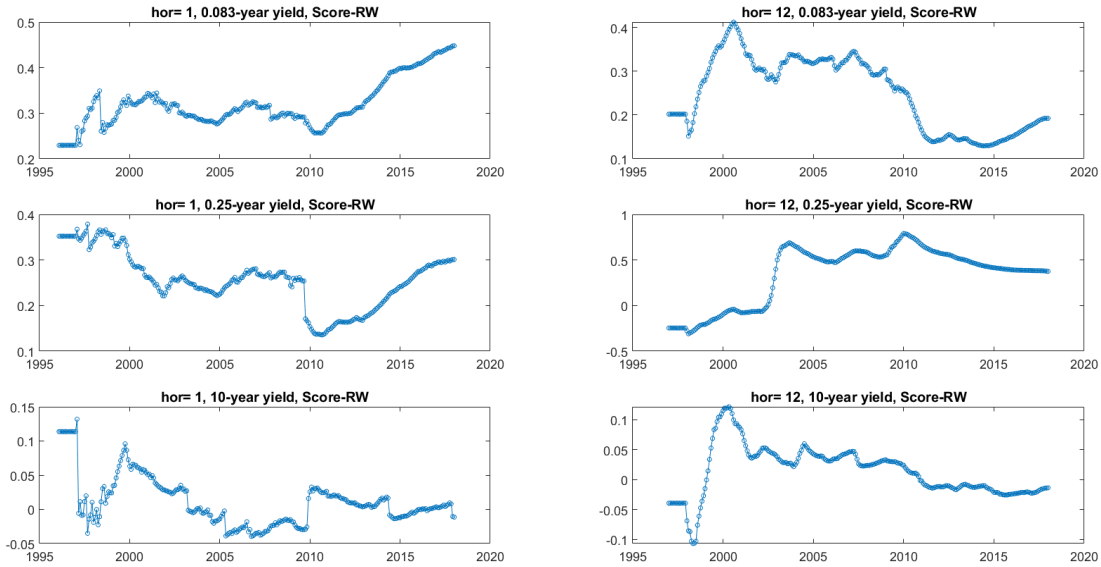
Figure 5: Figure 5: Recursive difference in SCORE of the JSZ-VAR-CSV versus the random walk. Recursive differences are computed starting from January 1996.
