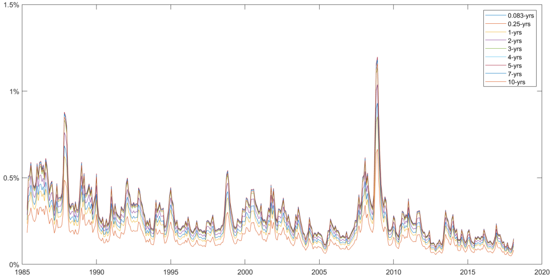
Figure 3: Volatilities for each yield (posterior medians)
