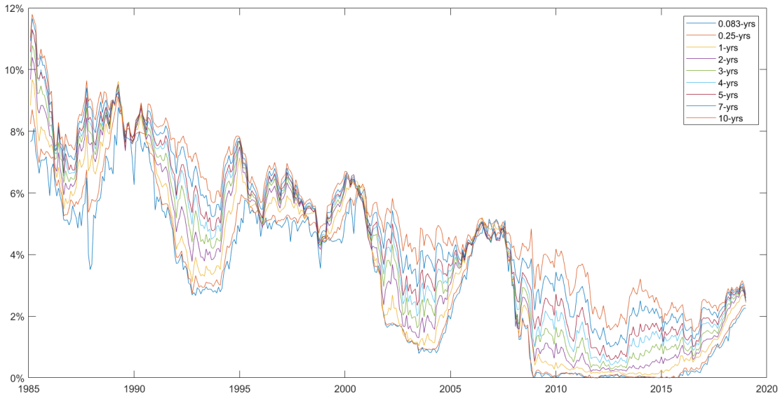
Figure 1: US zero coupon yields, Jan 1985-Dec 2018.
