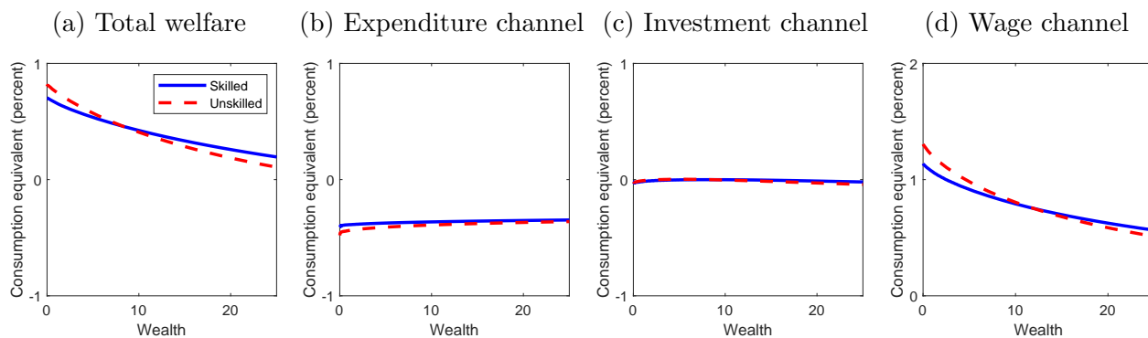
Figure 16: Welfare decomposition (labor income tax and no retaliation)
