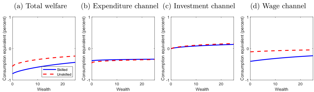
Figure 14: Welfare decomposition (no redistribution and no retaliation)
