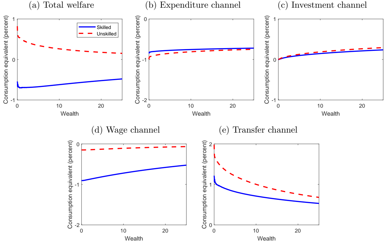
Figure 6: Welfare decomposition (lump-sum transfer and full retaliation)
