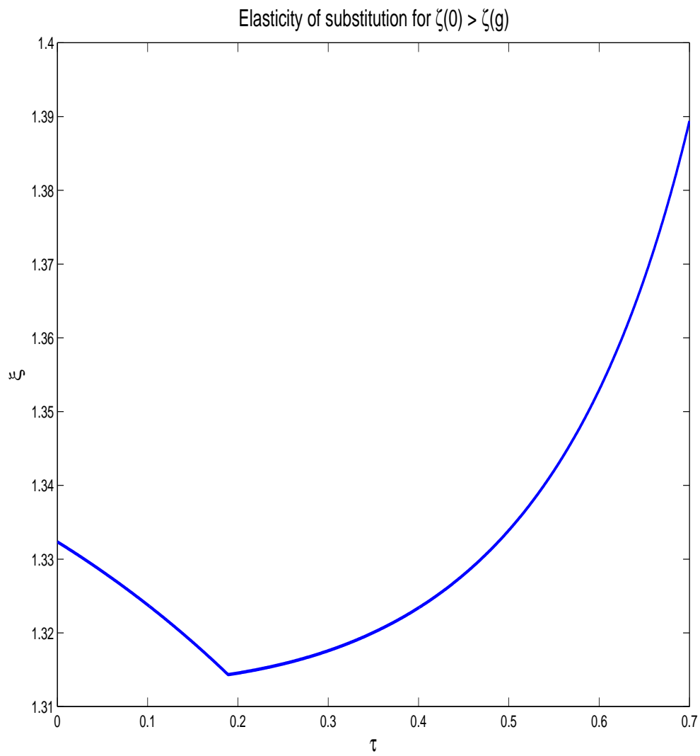
Figure 13: Necessary elasticity of substitution to cause higher inequality with zero growth
