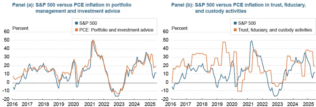
Figure 3: Correlation between S&P 500 and components of non-market-based PCE
