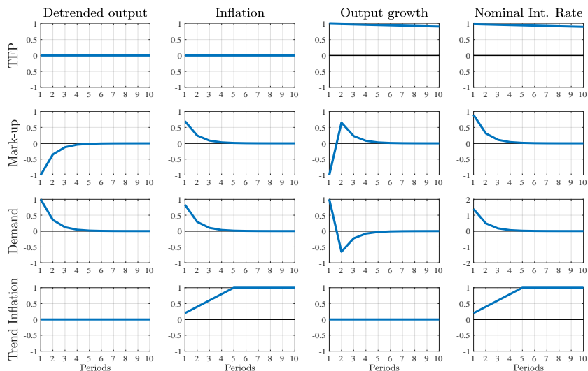
Figure 2: Selected impulse responses
